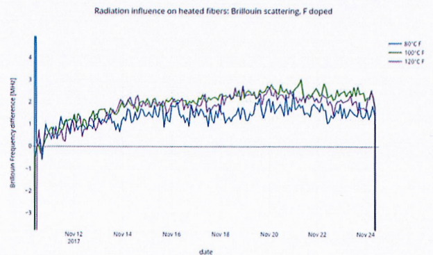
Brillouin frequency shifts of the F-doped fiber (1), for 3 heating temperatures, as a function of time (or irradiation dose)
