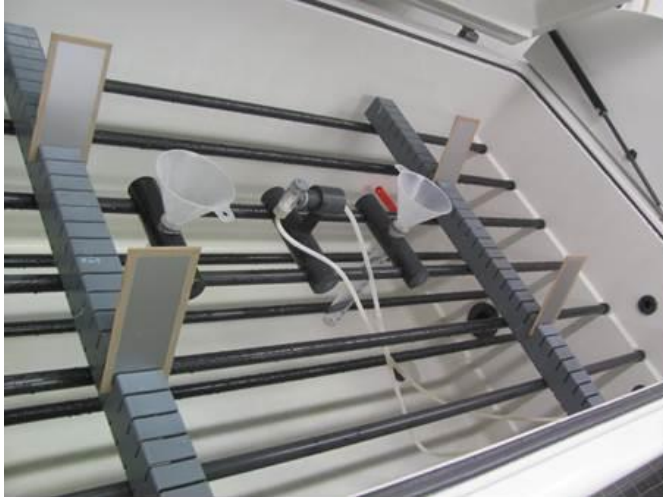
Figure of neutral salt spray(NSS) chamber calibration procedure
