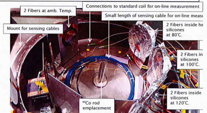
Picture of all the samples before the radioactive rod emplacement
