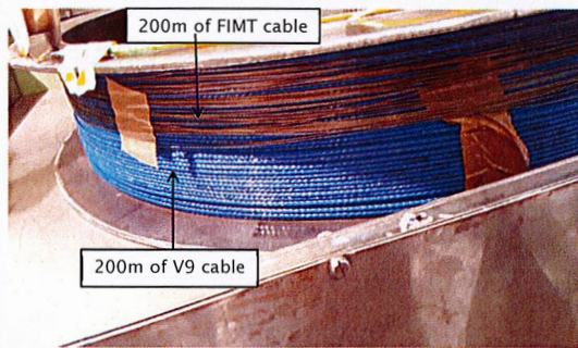
Optical fiber strain sensing cables (3) on their mount
