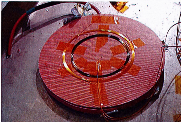
Inside view of one heating silicon with 2 enrolled optical fibers (1 and 2) and one thermocouple
