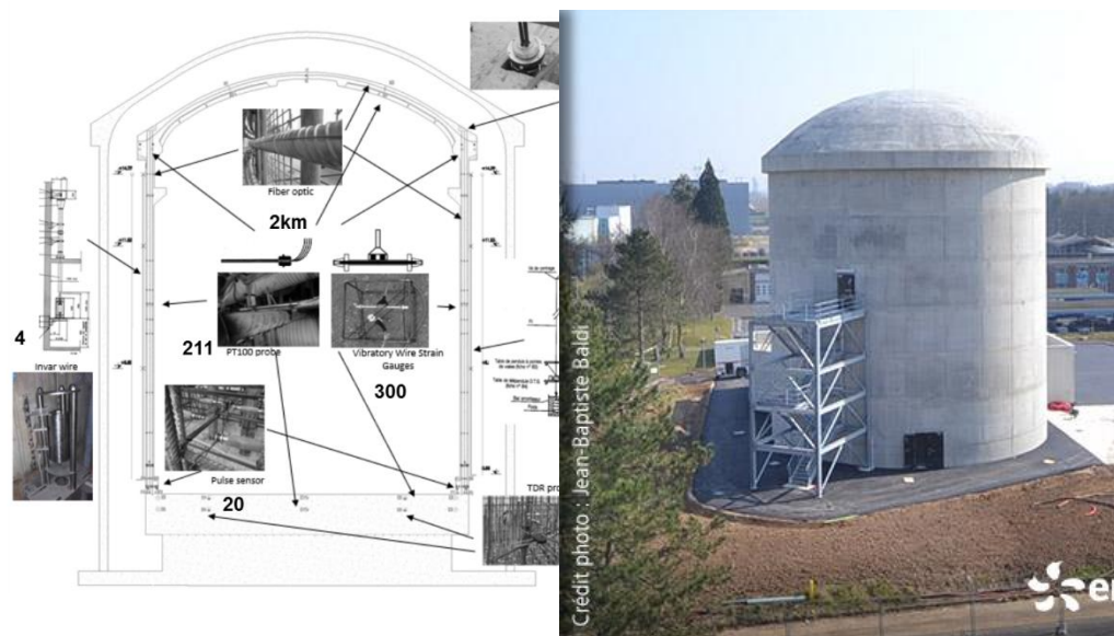
Figure 3-1: The VeRCoRs 1/3 scale-Mock Up: Comprehensive Monitoring System for Reduced Scale Containment Model – after an EDF conference paper 2016
