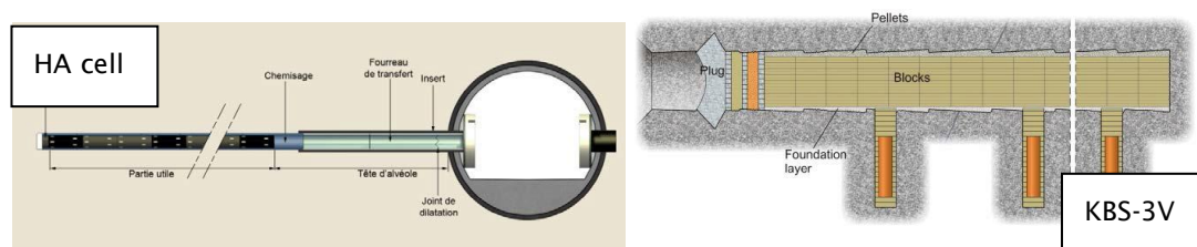
Figure 2-1: French (HA cell) and Swedish/Finnish (KBS-3V) concepts for High Level wastes discussed in this section
