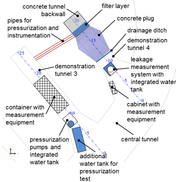
Figure 1. Top view of POPLU monitoring system arranged in demonstration tunnels 3 and 4, including pressurization system, leakage measurement system and data collection measuring equipment.
