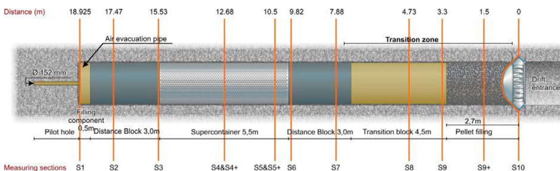
Figure 2. Schematic illustration of the MPT layout.
