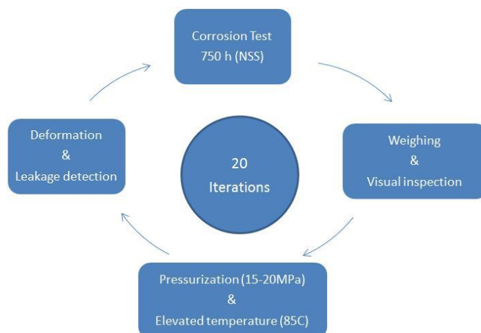
Figure 5-2: Cyclic robustness test concept diagram
