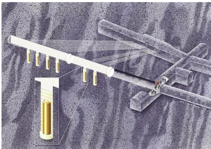
Figure 1. The layout of the Prototype Repository
