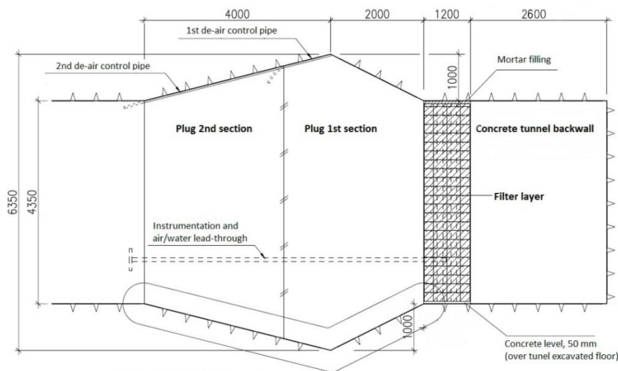
Figure 2: Schematic illustration of the Posiva's wedge-shaped plug being tested in POPLU
